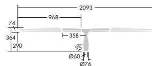
Double post top bracket
