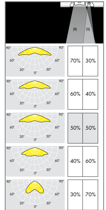
Fig. 2 The EQflux® system with intelligent driver, enables the factor to offer 15 pre-set light distributions by dynamically reconfiguring the LEDs. The standard pre-set settings of 50-50 is suitable for most applications.
