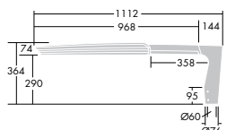
Scx 0.08m 2 Single post top bracket
