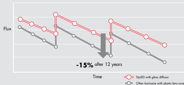
Comparison of the maintained flux characteristics of different enclosure materials: plastic is ageing while glass is steady
